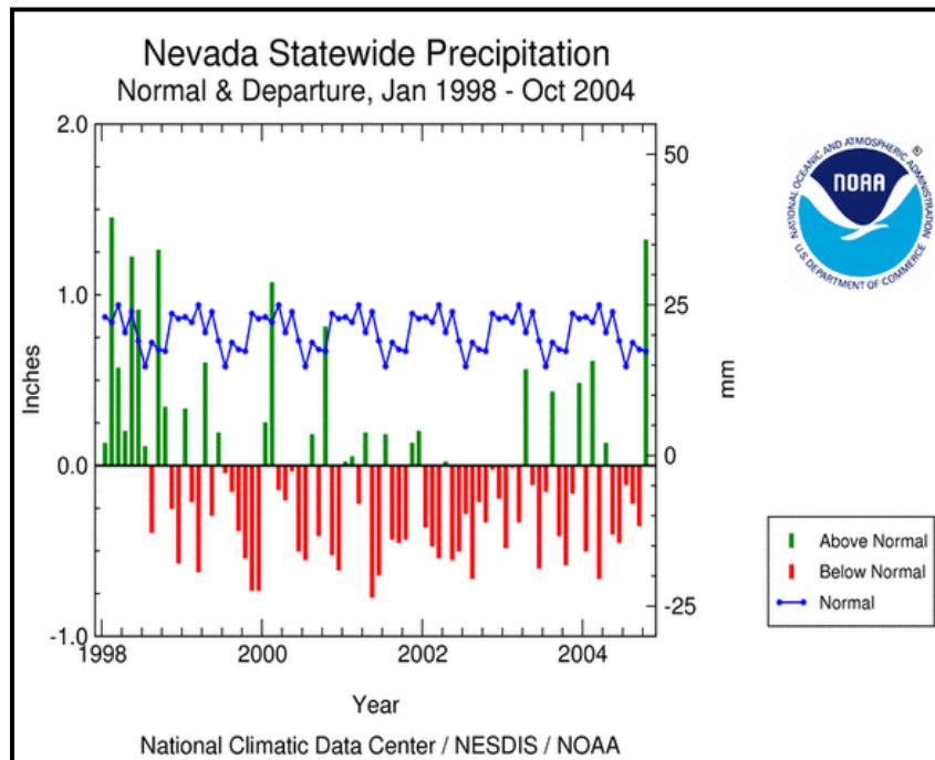
Figure 4-1. Nevada Statewide Precipitation, 1998-2005
