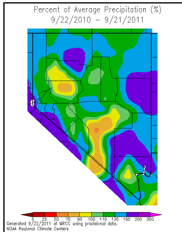
Figure 4-2. Percent of Average Precipitation, 2010 - 2011
