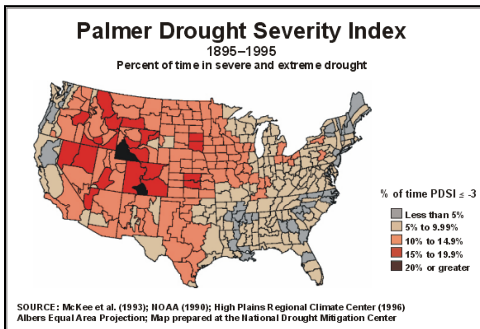
Figure 4-3. Palmer Drought Severity Index 1895-1995
